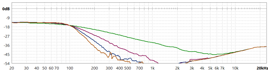
DSP Messung, Butterworth 6dB, 12dB, 18dB/octave 100Hz
